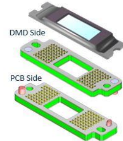
S315 Connector Shown
