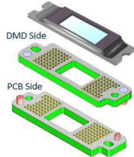
NCX S315 Connector Shown
