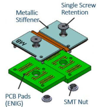
68 POS FX-Beam™ Termination
