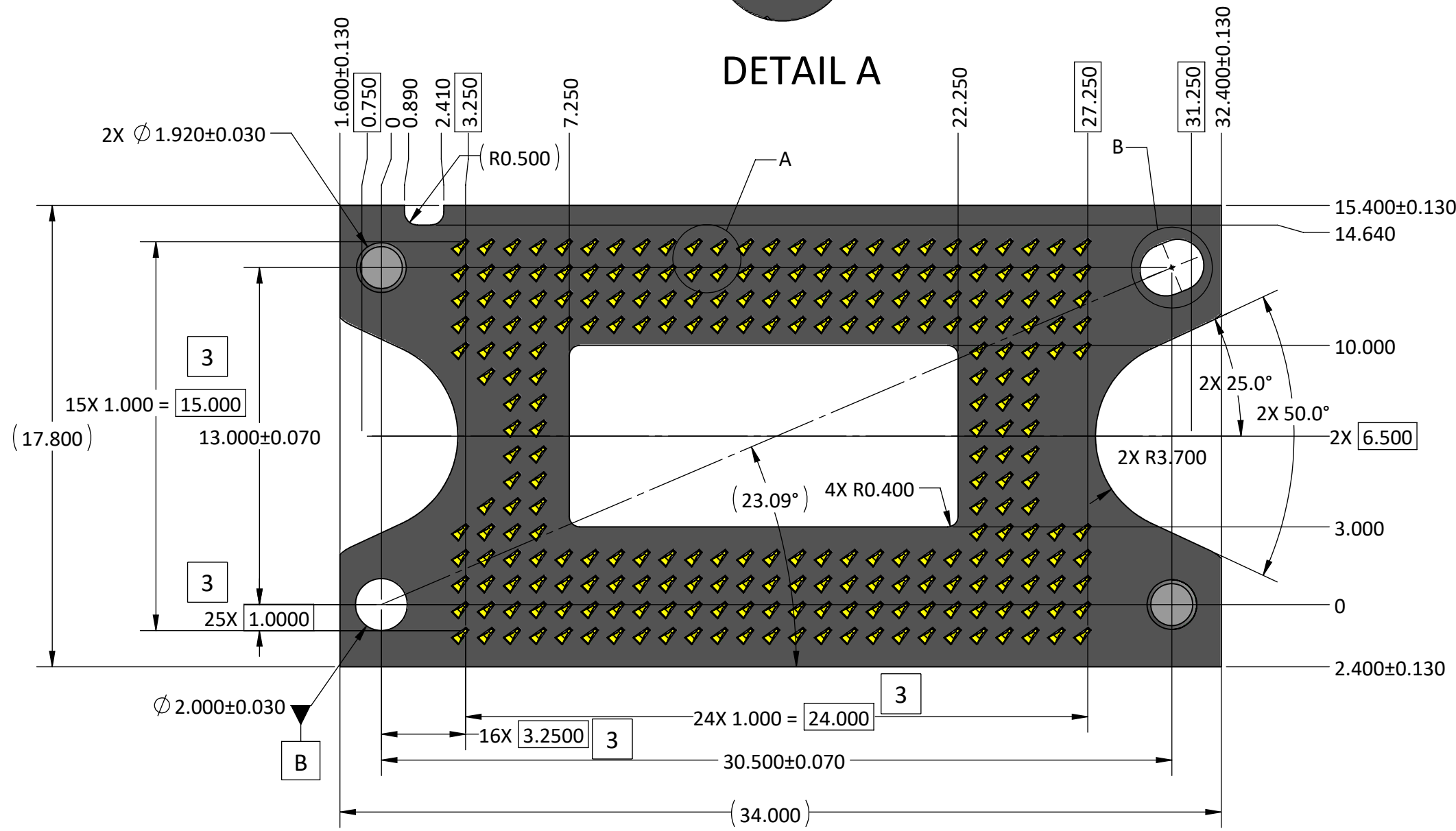
DMD LGA CONTACT SIDE
