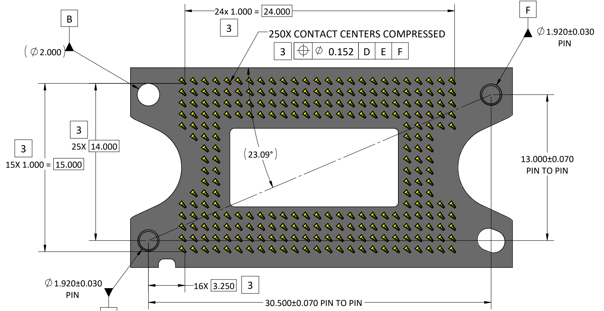
VIEW A -PCB LGA CONTACT SIDE
