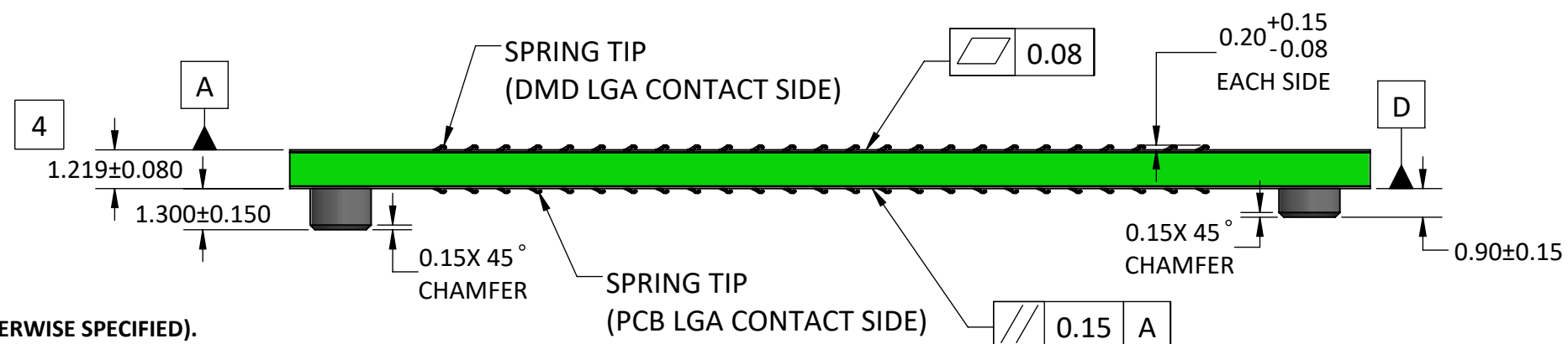
DMD LGA CONTACT SIDE
