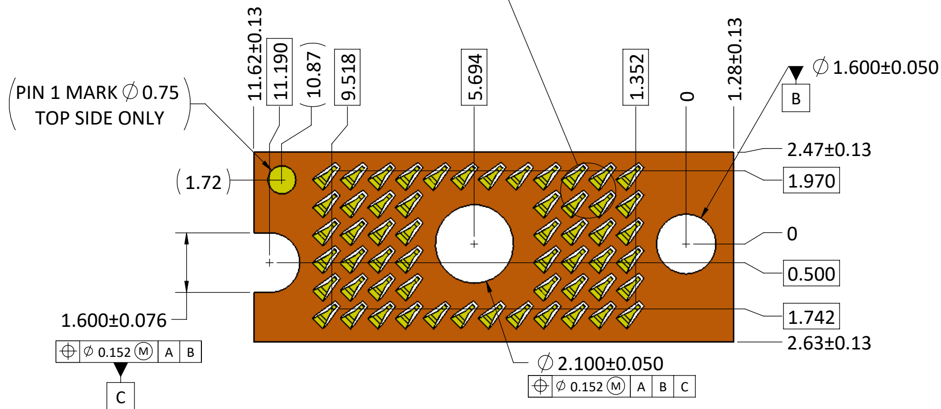
DETAIL B SCALE 20 : 1
