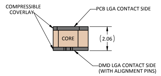
COMPRESSIBLE COVERLAY AND CORE
